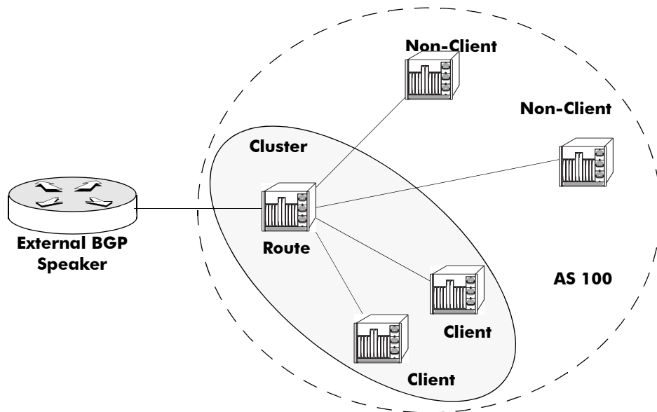
Route Reflector, Clients, and Non-Clients
